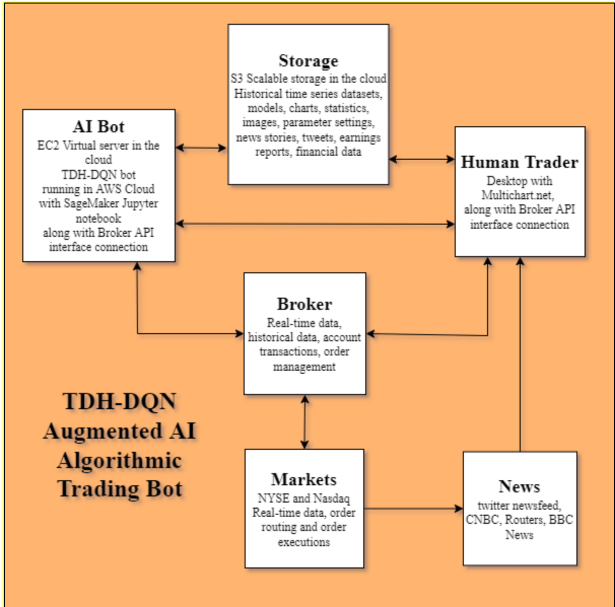
Figure 8. TDH-DQN Augmented AI bot Network Architecture
