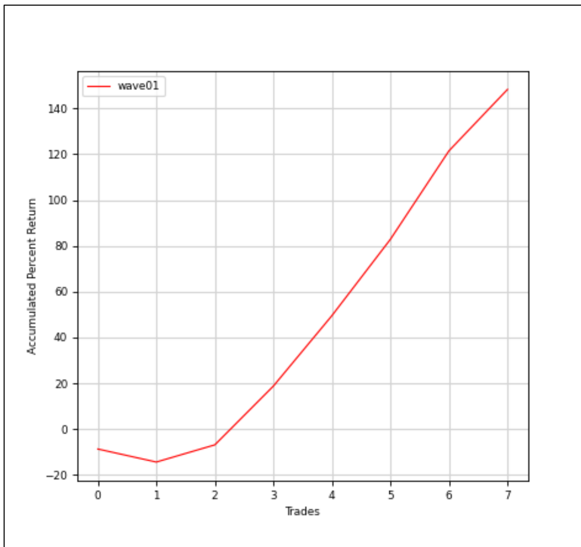
Figure 18. Part 3 Results: Shows the TDH-DQN bots APR for the Test Data.
