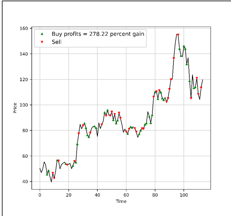
Figure A3. Part 2 AMD Price vs. Time Chart: TDH-DQN Swing Trading Bot's results.
