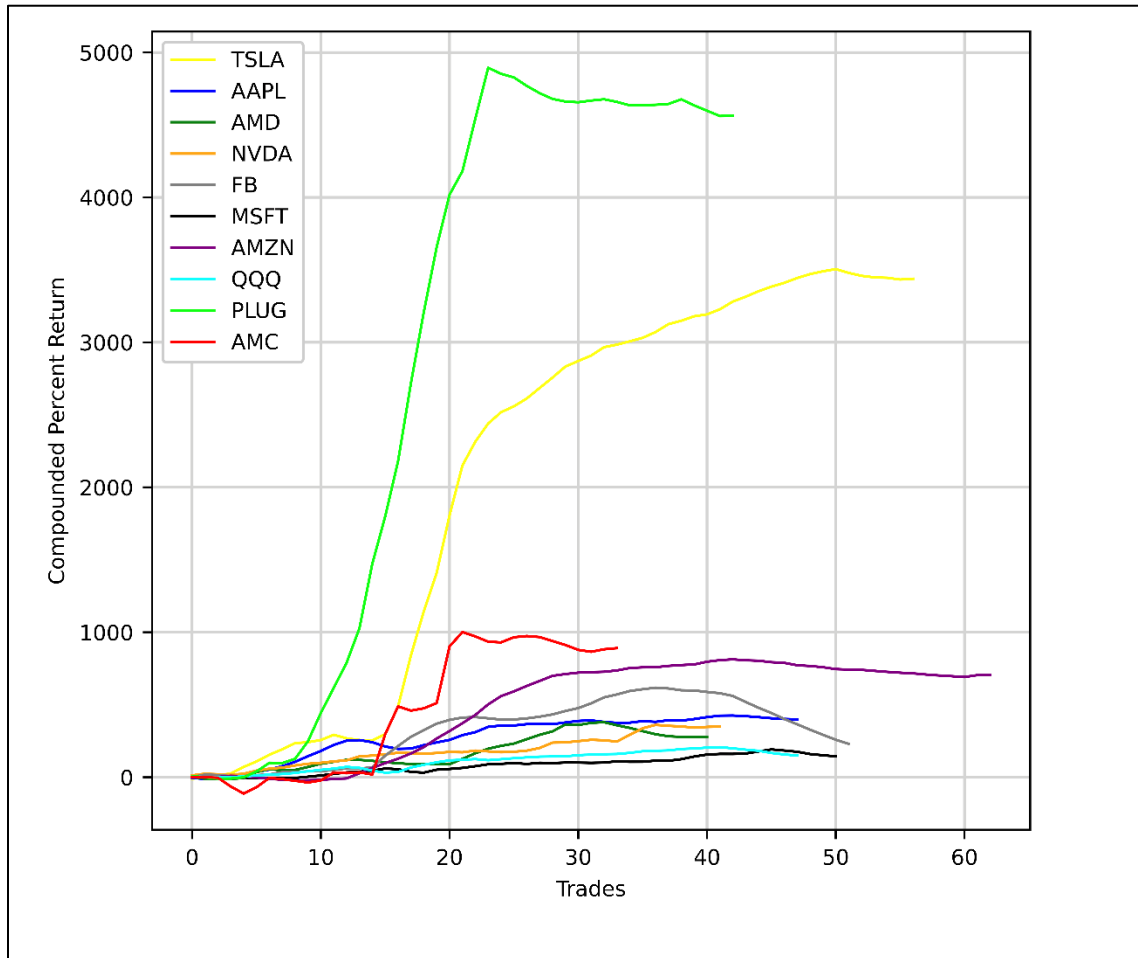
Figure 10. CPR vs. Trades for Part 2 TDH-DQN Bot Results from Table 13.
