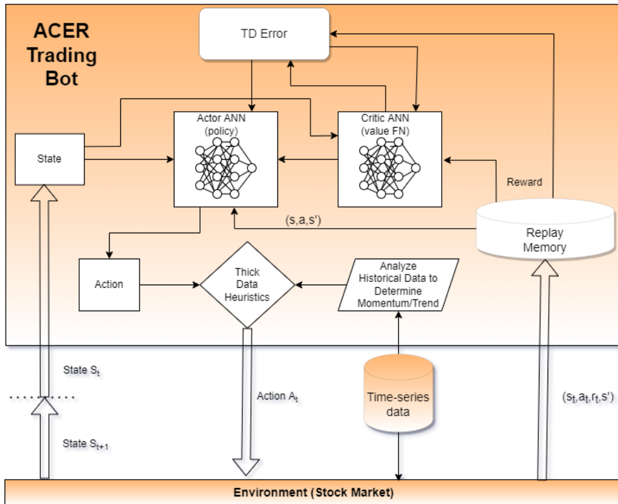
Figure 3. TDH ACER Trading Bot Architecture.
