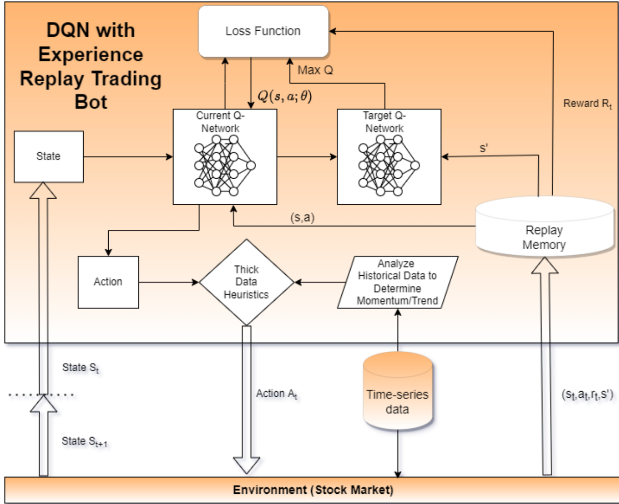
Figure 2. TDH-DQN Trading Bot Architecture.
