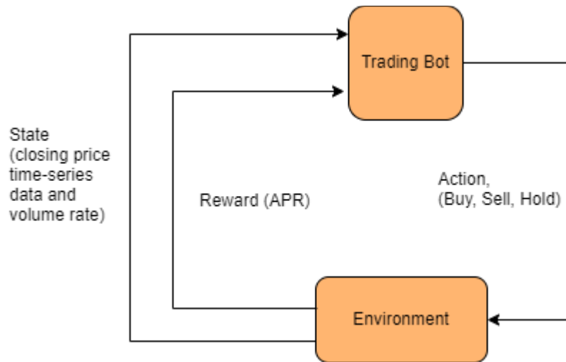
Figure 1.1. Trading Bot RL environment.
