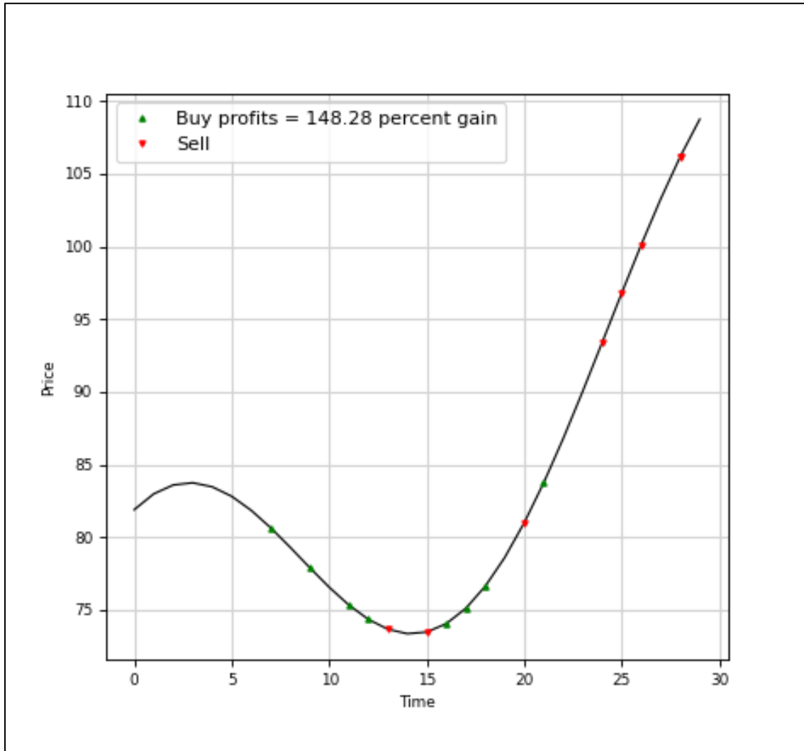
Figure 17. CPR vs. Trades for Part 3 Case Study Test Data Results.
