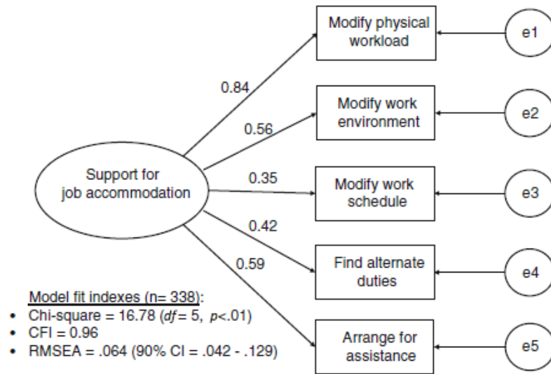
Figure 2. Results of the measurement model testing the goodness of fit among JAS factors to explain a central hypothetical construct of support for job accommodations.
