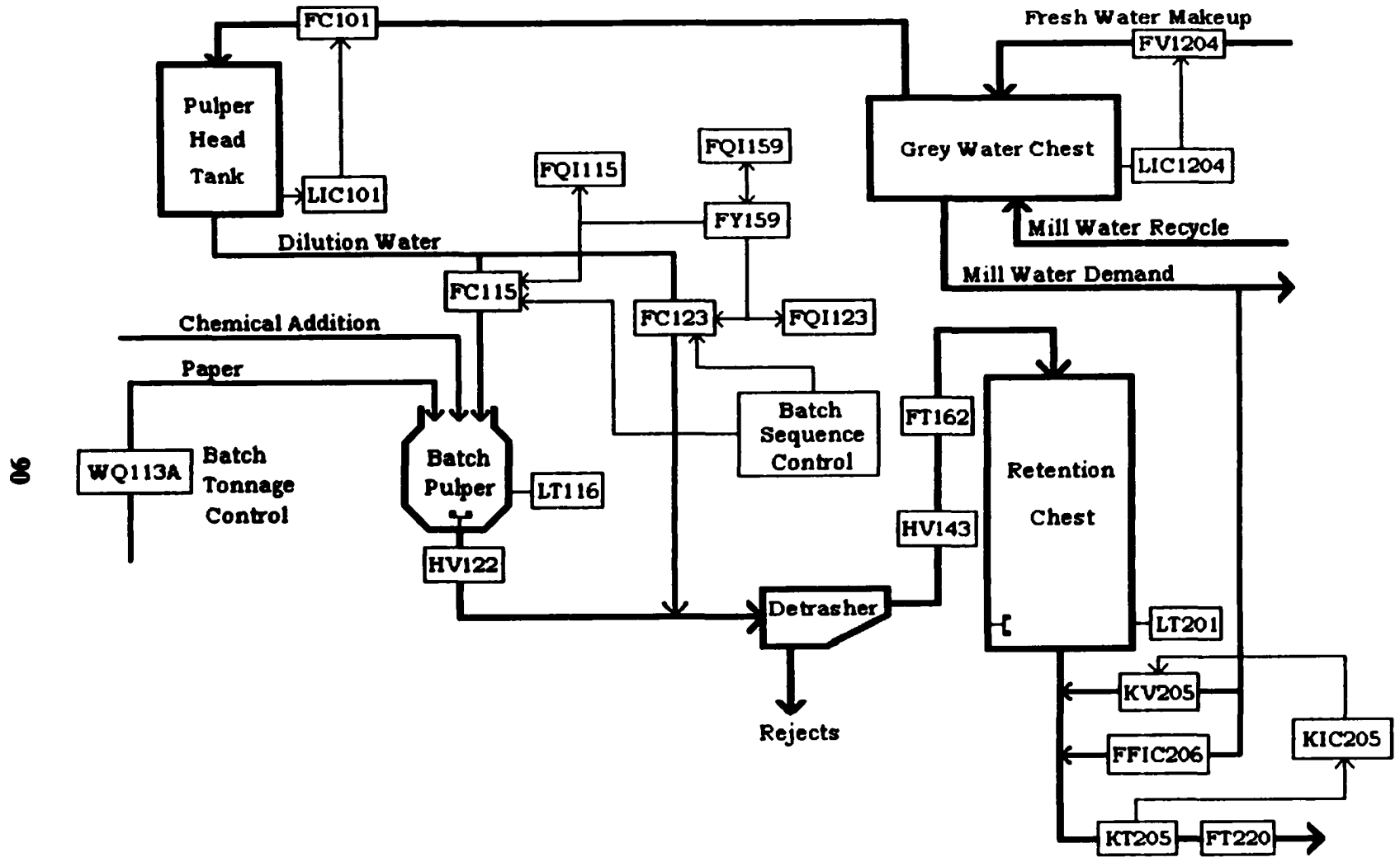
Figure 4.0 Pulper Discharge Process Flowsheet
