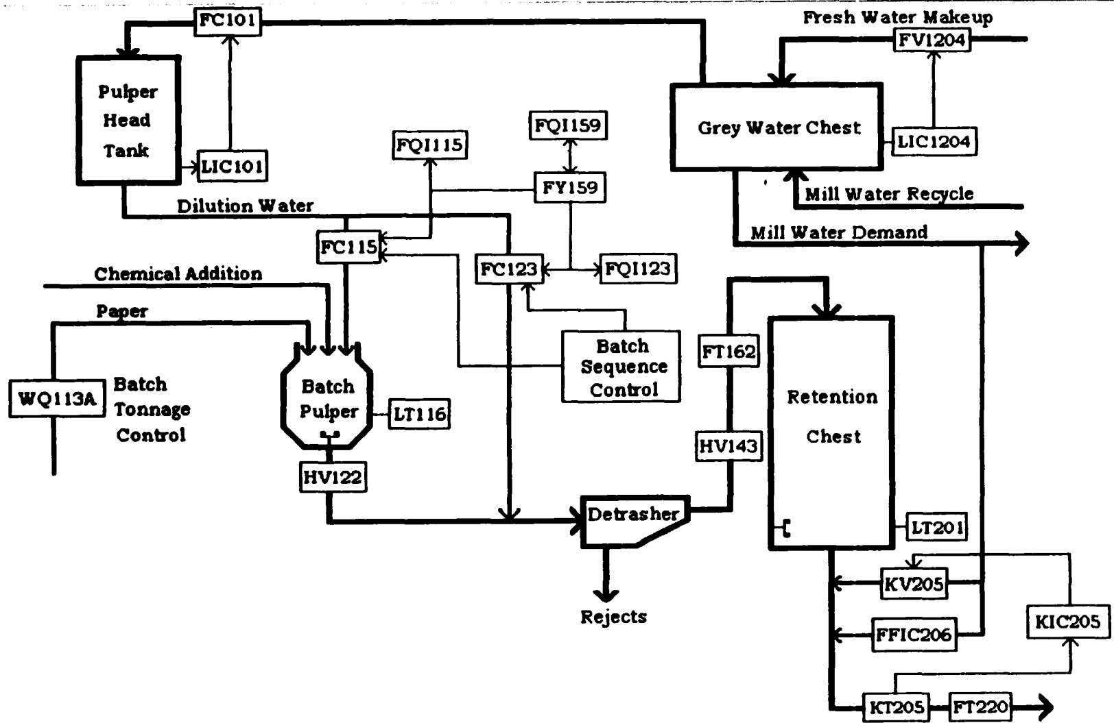
Figure 5.0 Grey Water Chest - Pulper Head Tank Control System
