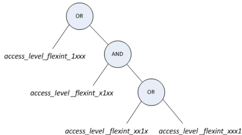
Figure 4.2: CP-ABE policy tree for access_level \geq 5
