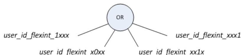
Figure 4.5: Access tree for user\_id \neq 4
