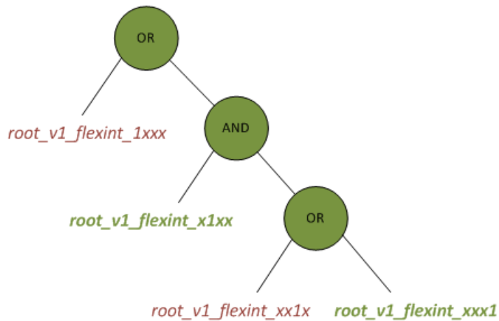
Figure 4.8: Policy tree requirement met by \text{USK}_{\text{Bob}} .
