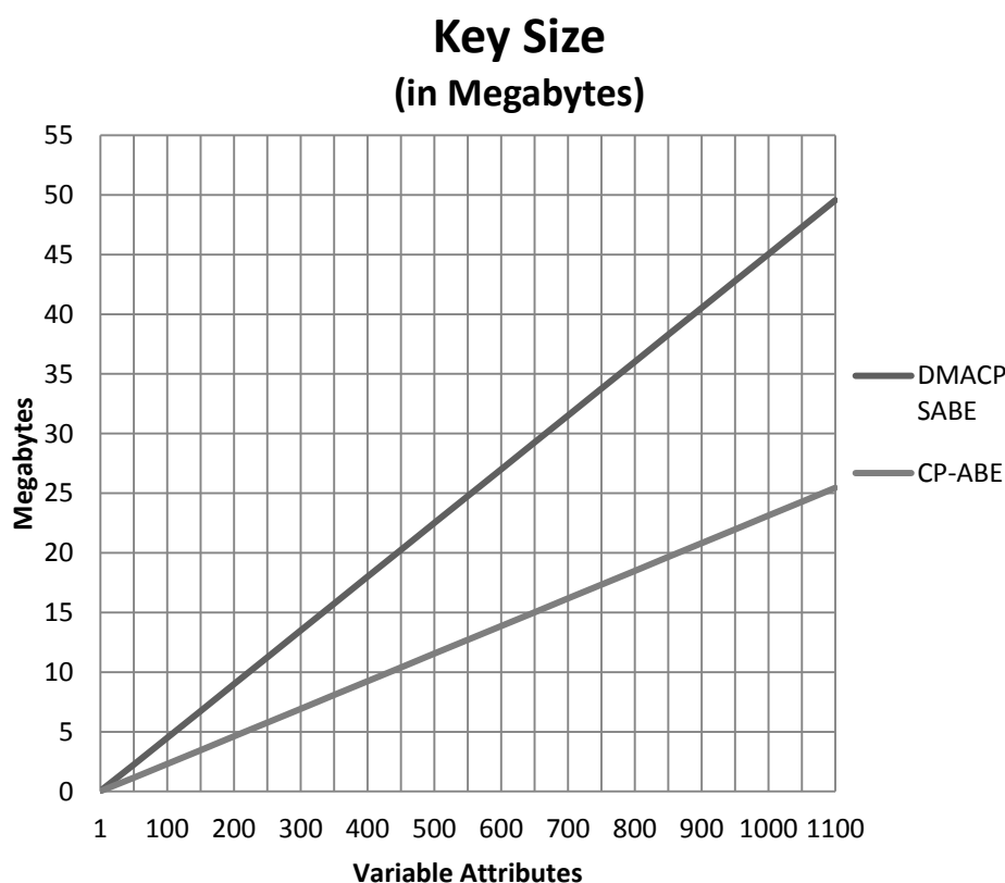
Figure 4.12: Size of a DMACPS ABE authority key vs. the size of a CP-ABE user key in megabytes for a \text{INT\_MAX} of 2^{64} .
