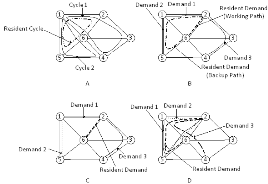
Figure 5.0.2: Including Resident Traffic: (A) Two cycles protecting an example network. One cycle that was used for the Resident Demand is also shown. (B) A resident demand and three new demands. (C) Working paths for the demands. (D) Backup paths for the demands. Note that the working and backup paths for non resident demands can be assigned to the resident cycle.
