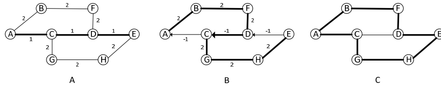
Figure 4.1.2: Finding Disjoint Paths With Modified Dijkstra Algorithm
