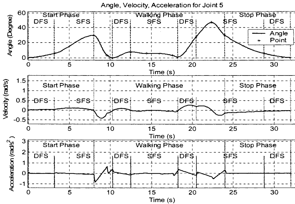
Figure 4-9 Angle, Velocity and Acceleration for Joint 5
