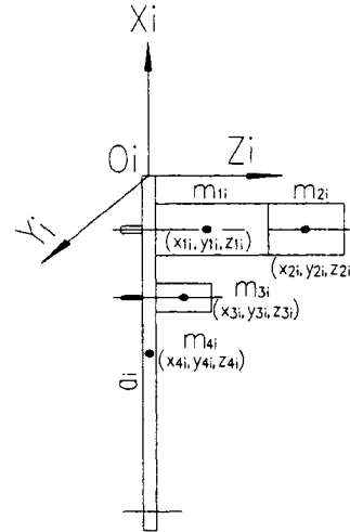
Figure 5-1 Link Structure
