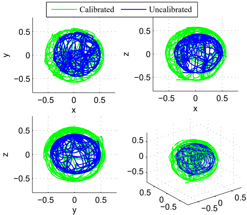
Figure 3.12: Magnetometer calibration results
