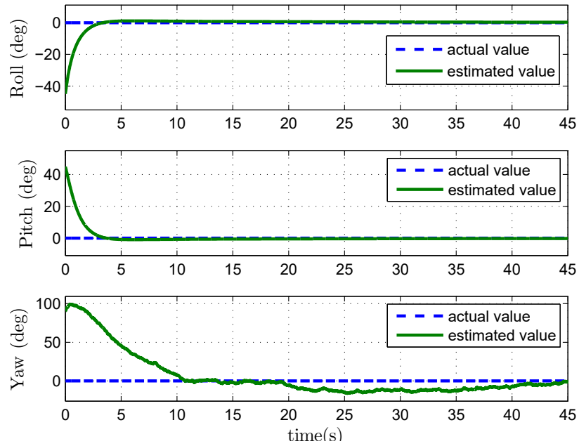
Figure 4.1: Static attitude estimation with gyro-bias
