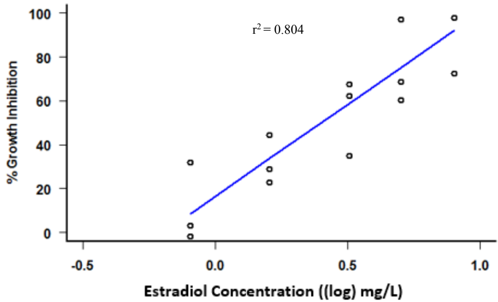
Figure 2.25 - Semi-log scatter plot of 17-b Estradiol concentration and percentage inhibition of growth for Asterionella formosa using regression analysis.
