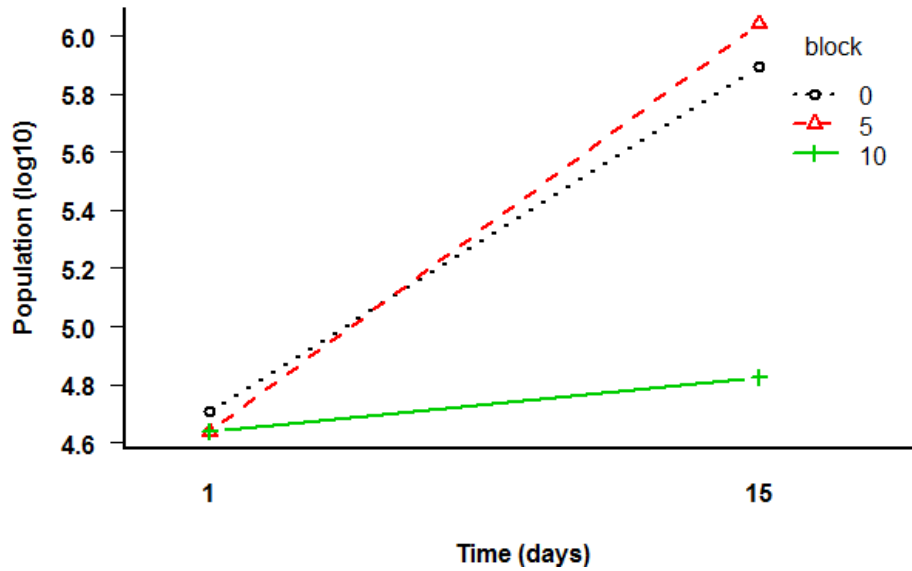
Figure 2.19 - An illustration of a Blocked ANOVA depicting changes in cell density of Diatoma tenuis with 17-β Estradiol over the course of the second trial.
