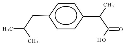
Figure 1.2 – Benzeneacetic acid, \alpha -methyl-4-(2-methylpropyl).
