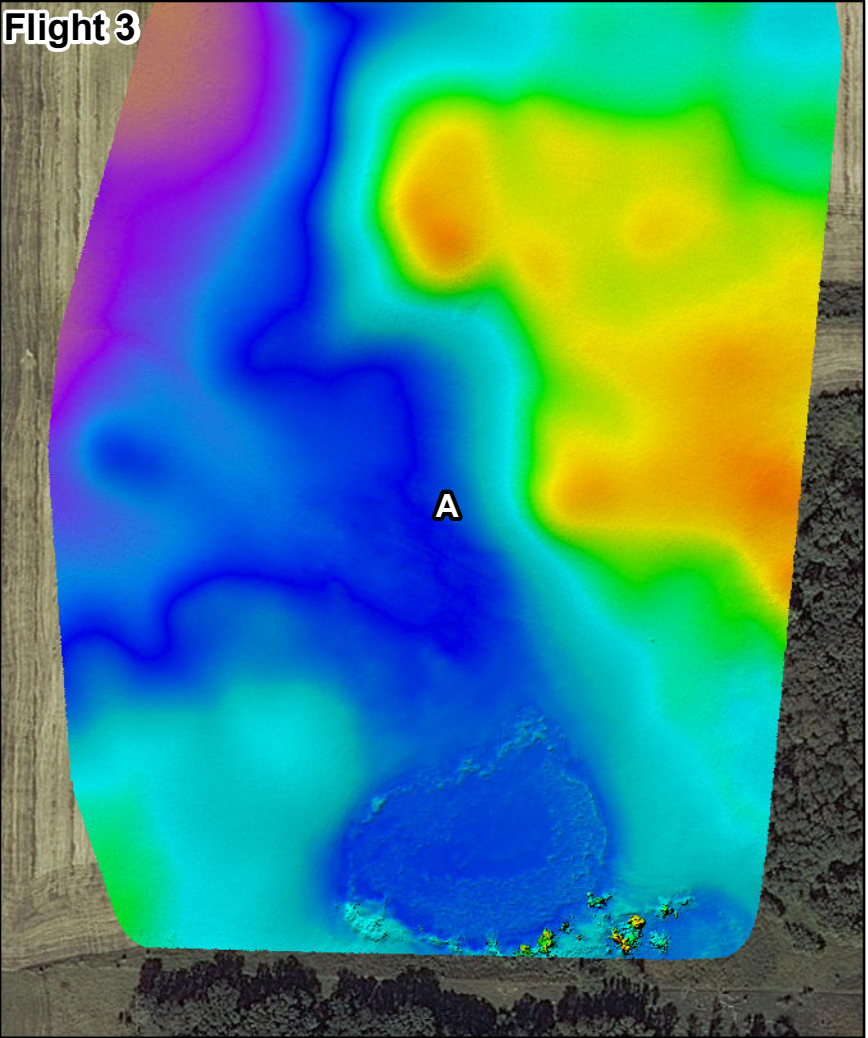
Figure 4-34: Raster DEMs
