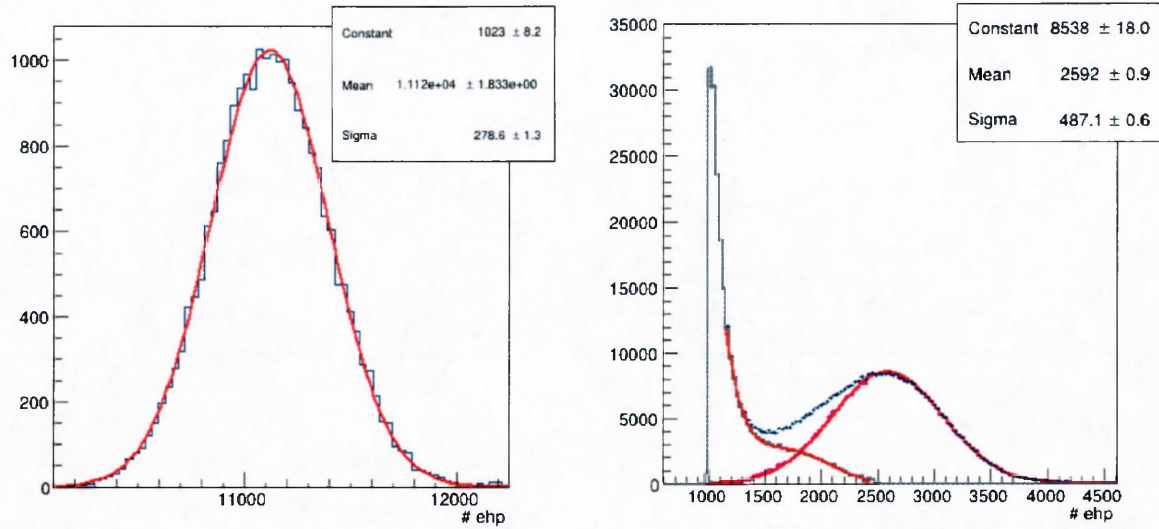
Figure 3.23 The electronics noise attributed to the pulser signal, shown on the left, and the noise in the total PHS signal is fitted in red, for the PHS measurement of 30 V/ \mu\text{m} . Assuming the electronics noise does not cross the \langle n_0 \rangle of the total signal, this can be fitted to give the width of the electronics signal, \sigma_e , and total signal, \sigma_0 , to acquire the intrinsic noise, \sigma_i . The noise peak is fit to a Poisson function and the pulser and photopeak to a Gaussian.
