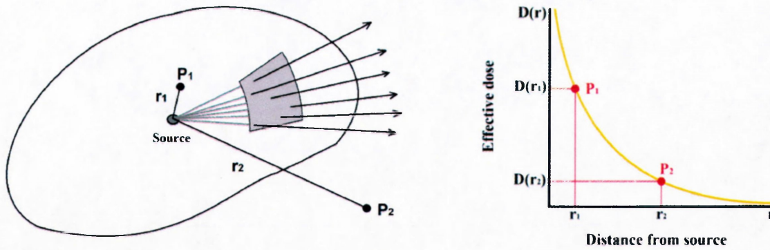
Figure 1.4 The left image illustrates the isotopic photon emissions from the brachytherapy source at two points: P_1 and P_2 . At a distance, r , the effective dose, D(r) , decays by the inverse square law, shown graphically on the right.
