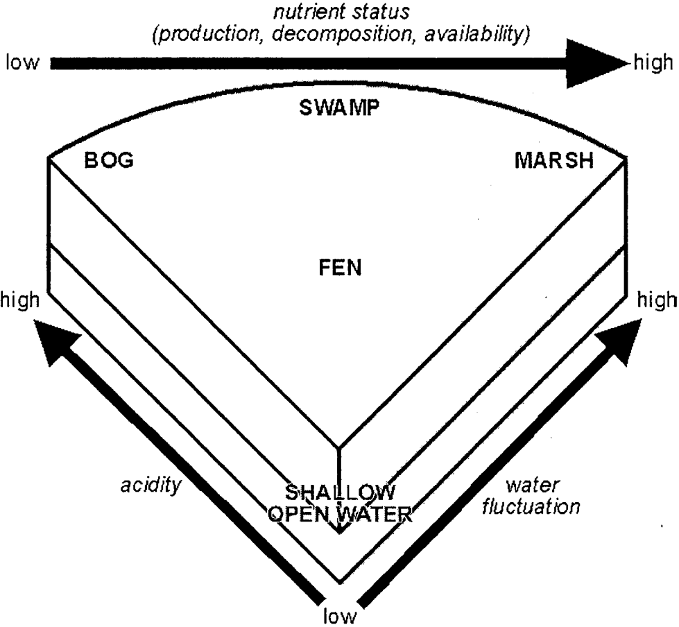
Figure 2. The five classes of the Canadian Wetland Classification System (indicated by capital letters) relative to important gradients. Water level fluctuation and acidity should be interpreted as distance from the origin. Modified from Zoltai and Vitt (1995).
