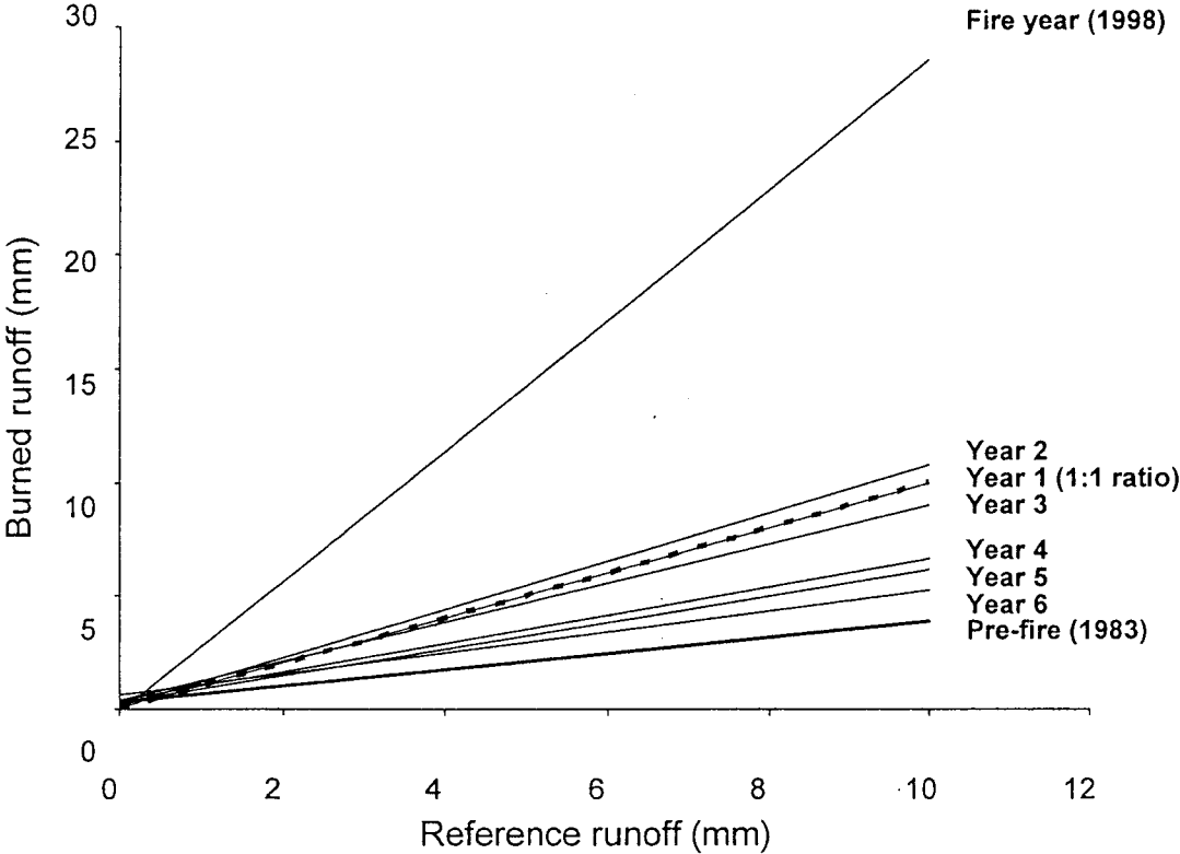
Figure 3-5 Regression lines between total daily runoff from the large burned and large reference watersheds for the pre-fire year, fire year and Years 1 through 6 post-fire. Relationships are based on 12 to 101 data points per year. A 1:1 ratio between the burned and reference watersheds indicated by dashed line.
