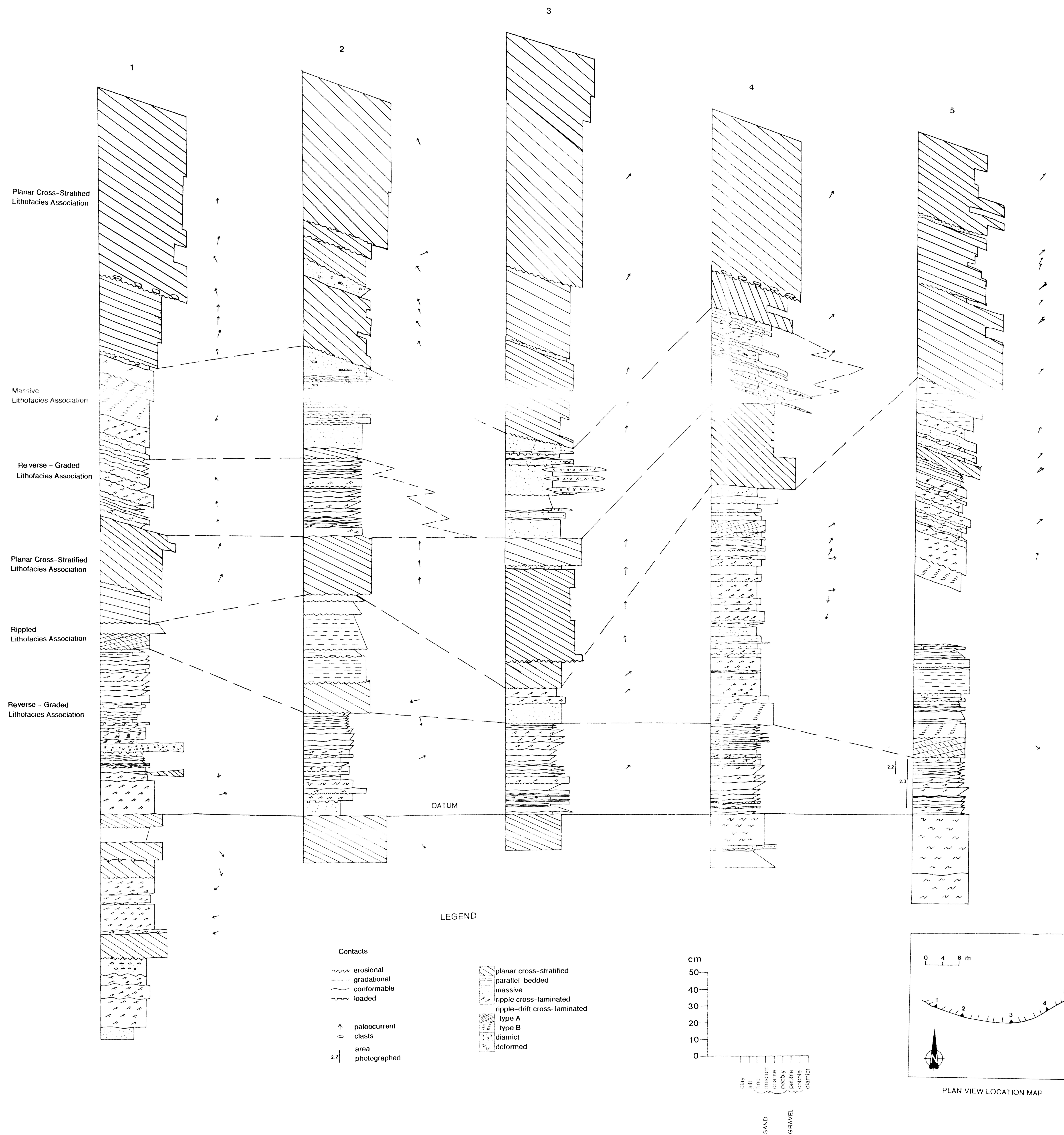
FIGURE 2.1 BEARDMORE DETAILED STRATIGRAPHIC SECTIONS
