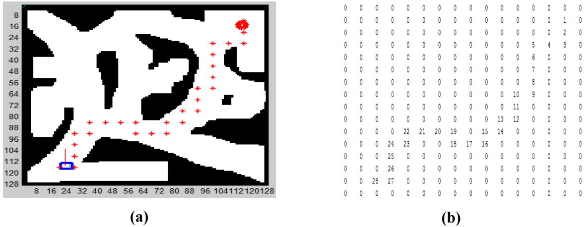
Figure 4-6: (a) A-Star path plotted. (b) The corresponding matrix to the path.
