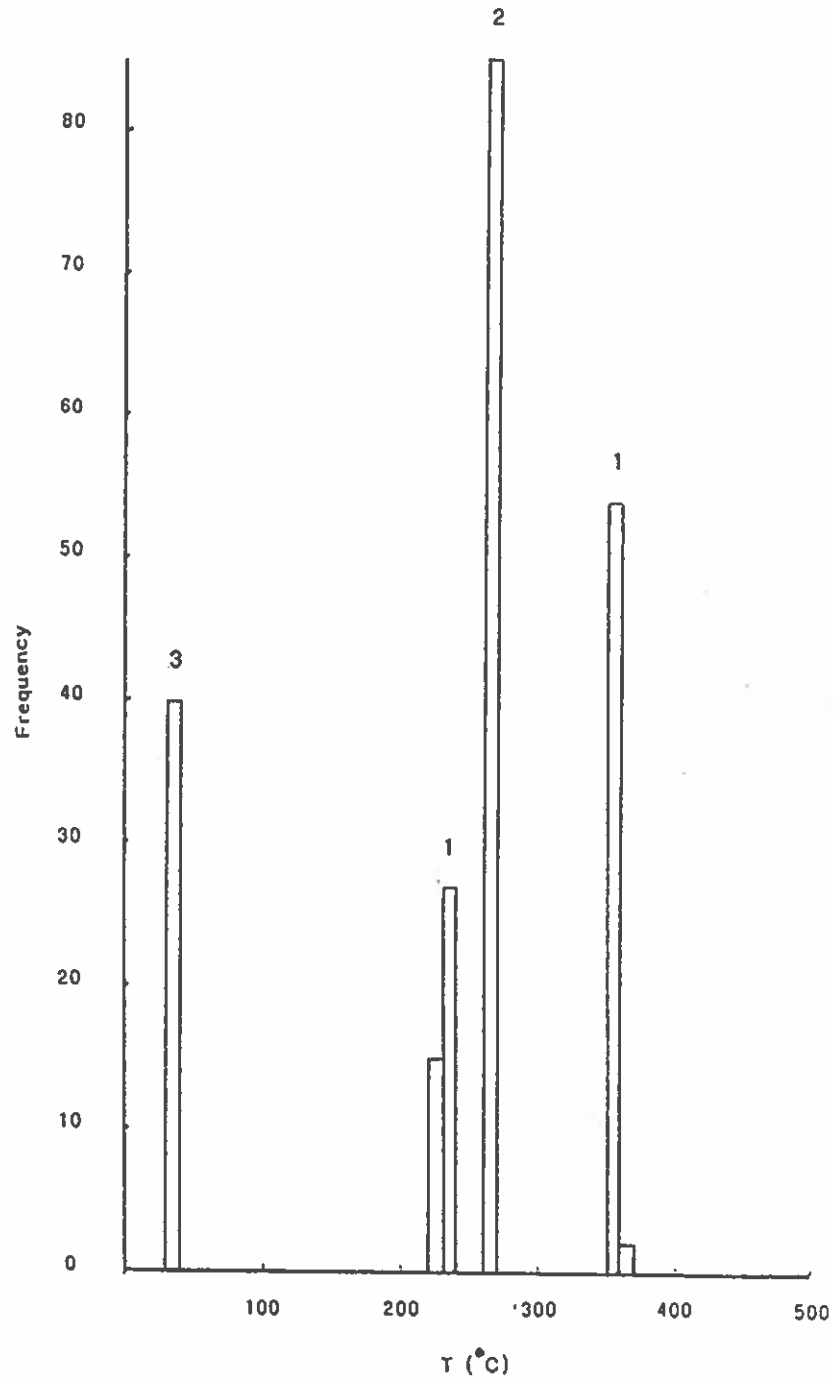
Figure 4-5: Homogenization temperature data from Metalore Stages 1, 2 and 3.
