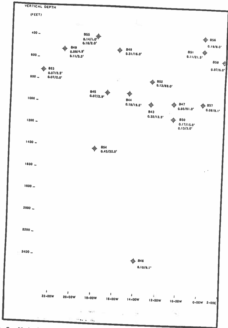
Figure 2-2: Metalore Contact Zone long section, looking north, ⊕B43 indicates the diamond drill hole number and 0.32/12.3' represents 0.32 ounces of Au per ton across 12.3 feet.
