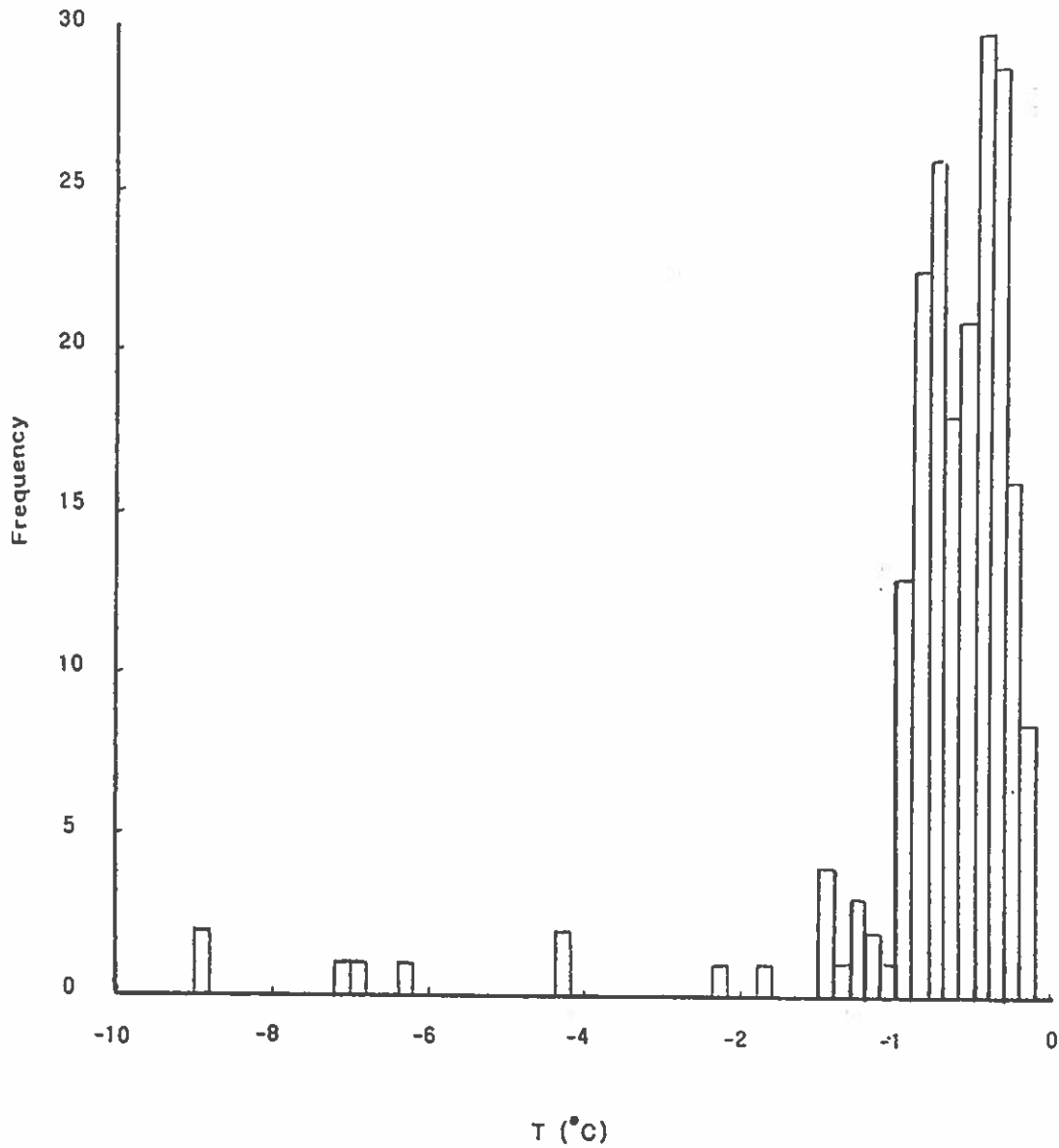
Figure 4-4: Final melting temperature data from Metalore Stages 1, 2 and 3. There are no apparent groups of data for each stage of mineralization.
