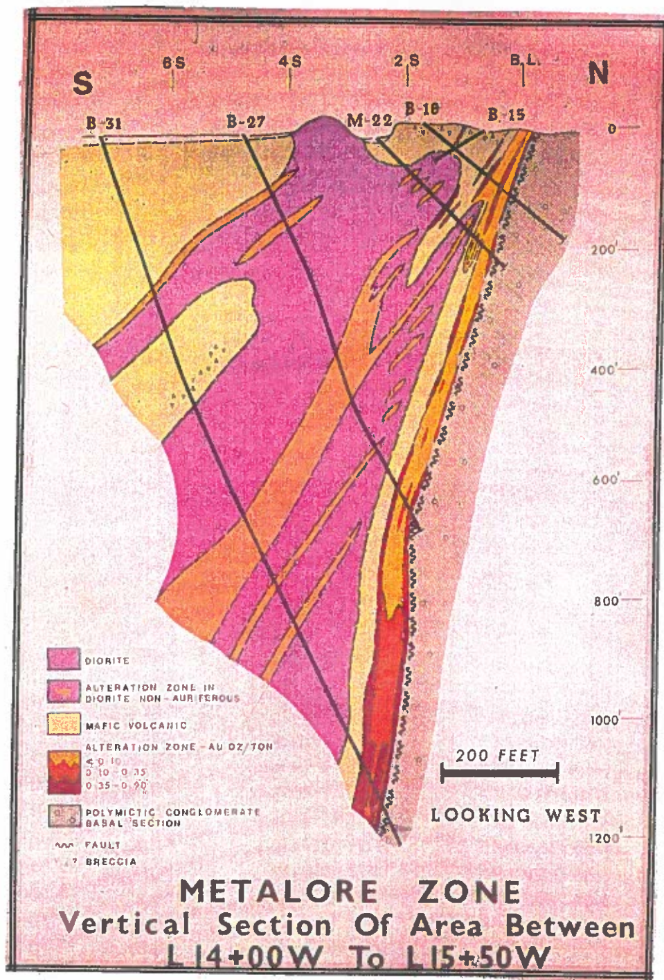
Figure 2-3: Vertical section of the Metalore zone showing the alteration and ore zone at depth, whereas, thin, erratic lenses of the alteration occur toward surface. Also shown is the barren alteration zone in the dioritic rocks. The black lines depict diamond drill holes with their drill hole numbers at surface.
