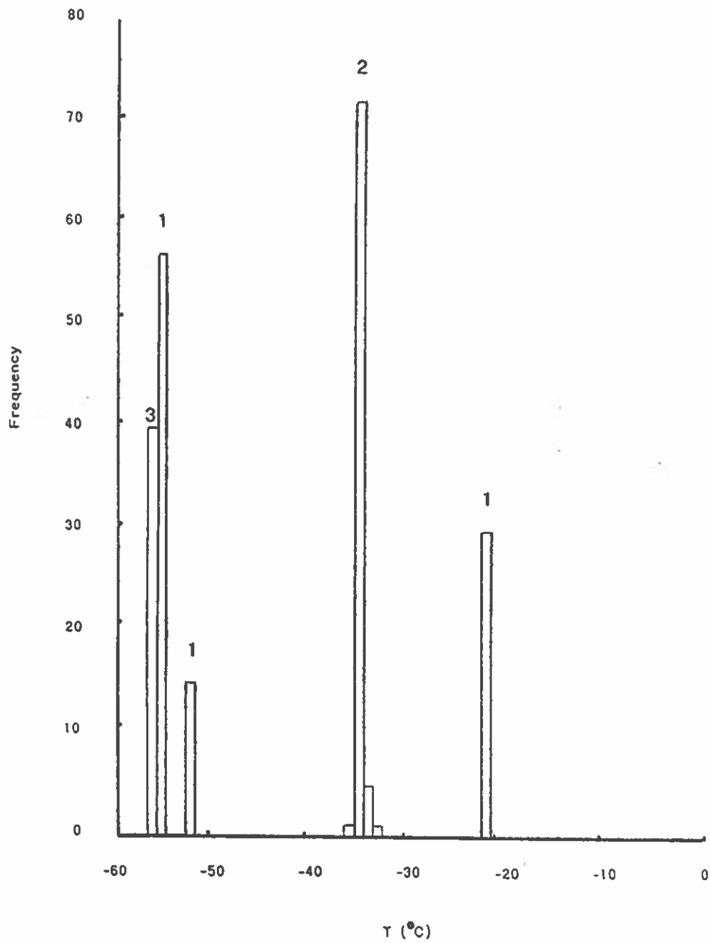
Figure 4-3: Eutectic temperature data from Metalore Stages 1, 2 and 3.
