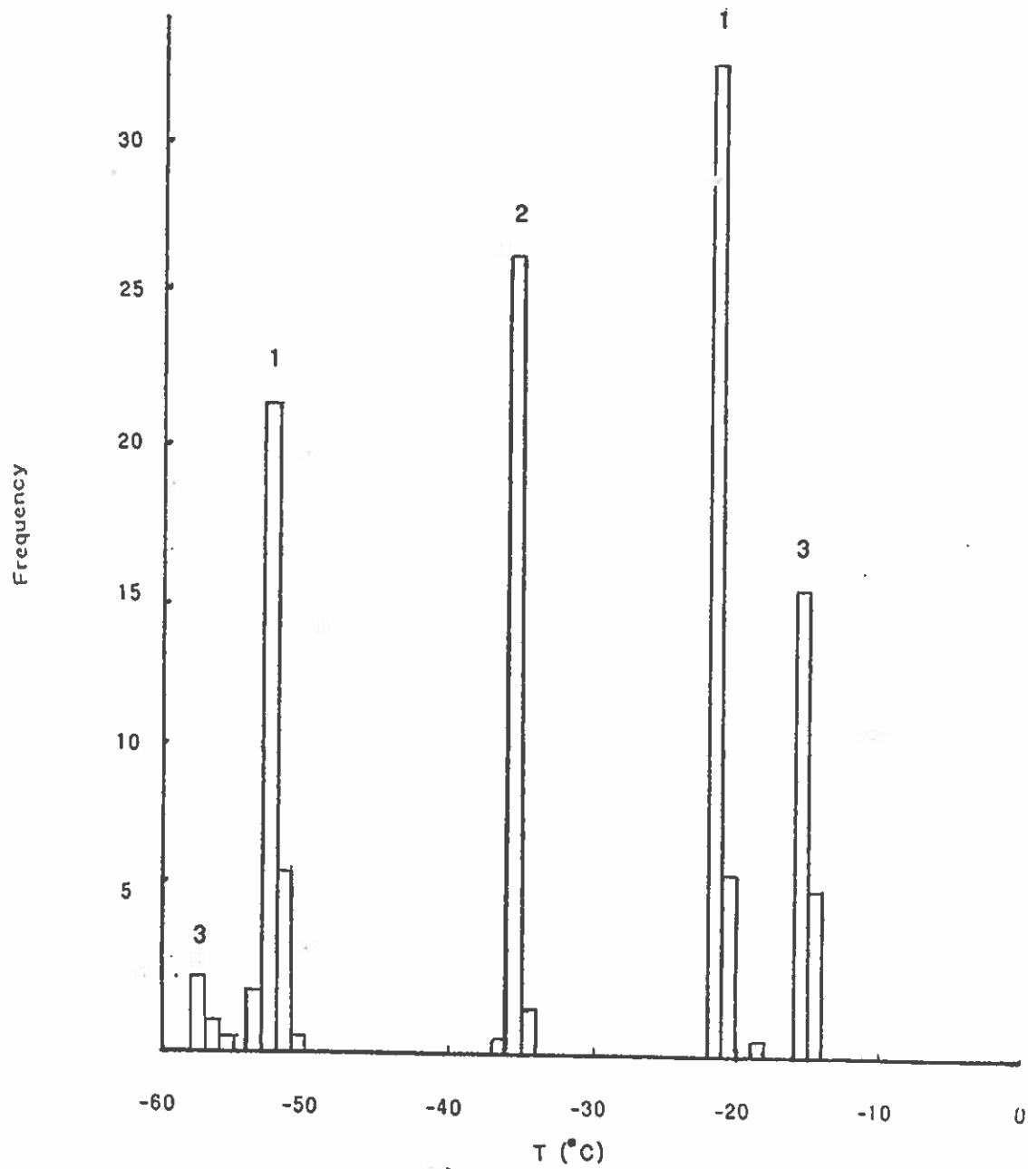
Figure 4-1: Eutectic temperature data from Golden Highway Stages 1, 2 and 3.
