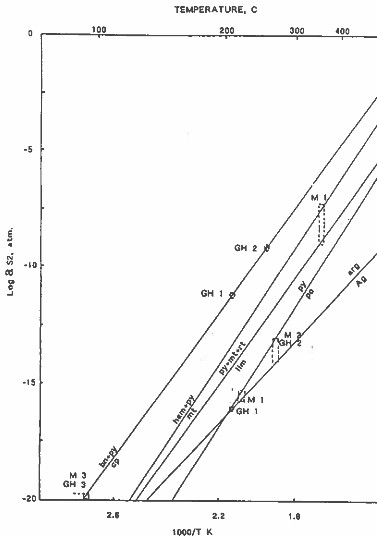
Figure 5-1: Mineral paragenesis, homogenization temperatures and activities for sulphur in the Metalore (M) and Golden Highway (GH) during Stages 1,2 and 3 indicated by M1, M2, M3 and GH1, GH2 and GH3 respectively. The minerals occurring in these stages are hematite (hem), pyrite (py), magnetite (mt), rutile (rt), ilmenite (ilm), argentite (arg), pyrrhotite (po), bornite (bn) and chalcopyrite (cp).
